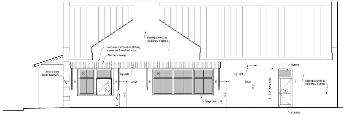
02 Proposed North Elevation 1/4" = 1'-0"
